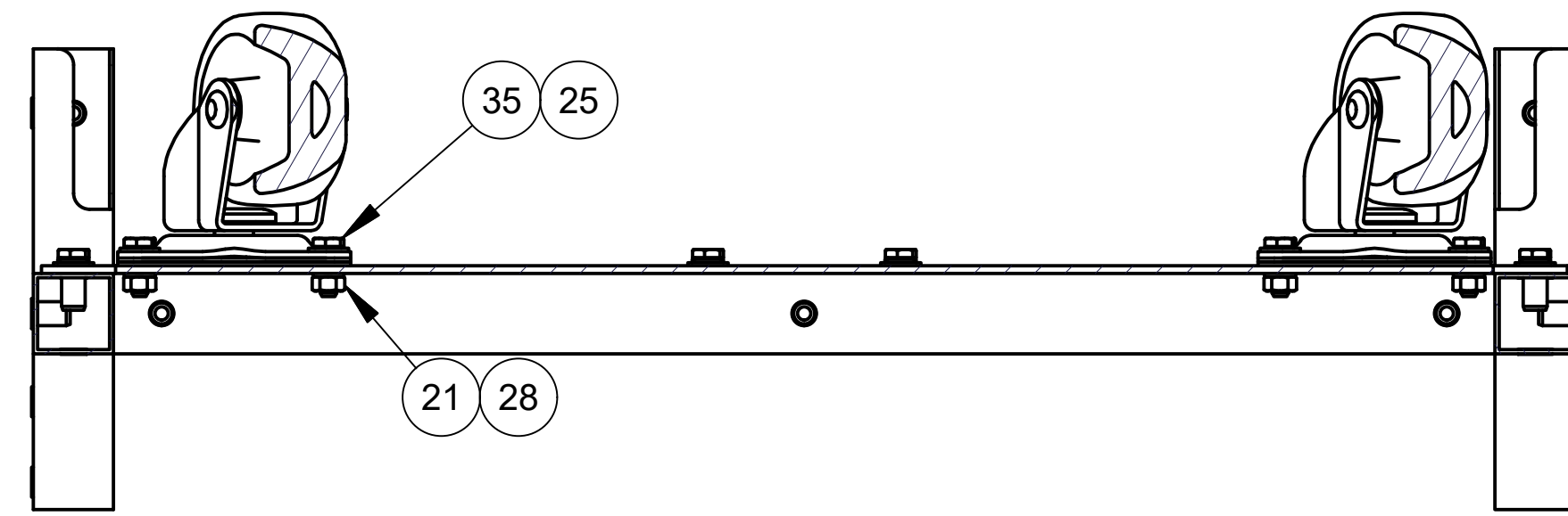
SECTION B-B
