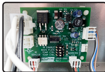
Diagnostic And Temperature Control Circuit Board
